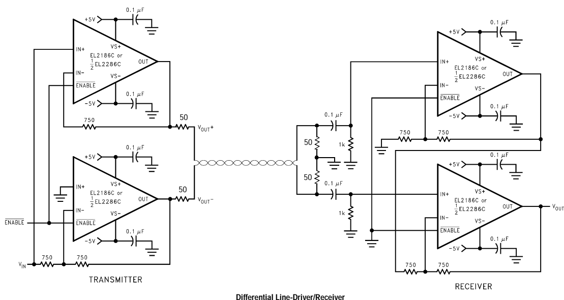
Differential Line-Drive/Receiver
