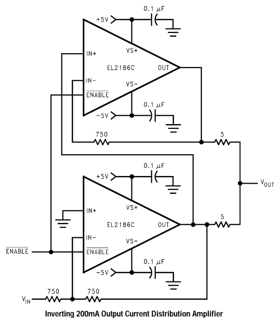
Inverting 200mA Output Current Distribution Amplifier
