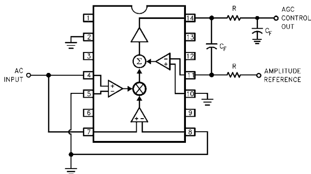
FIGURE 2. SIMPLIFIED AGC DETECTOR/DC FEEDBACK CIRCUIT
