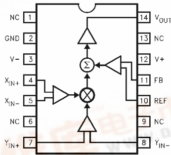
EL4450 (14-PIN PDIP, SO) TOP VIEW
