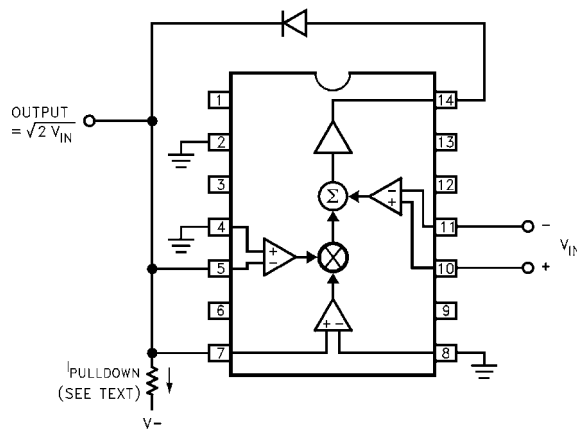
FIGURE 5. SQUARE-ROOTER
