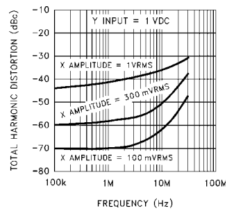
Total Harmonic Distortion of X Input vs Frequency
