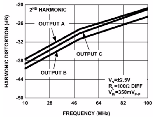
FIGURE 30. HARMONIC DISTORTION
