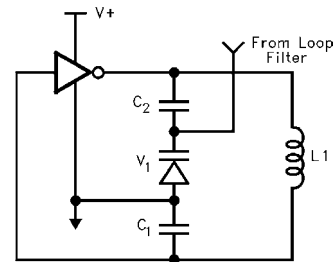
COLPITTS OSCILLATOR
