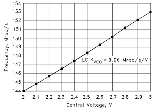
FOSC vs VC, LC VCO
