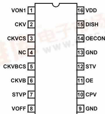
EL5000A (16-PIN TSSOP) TOP VIEW
