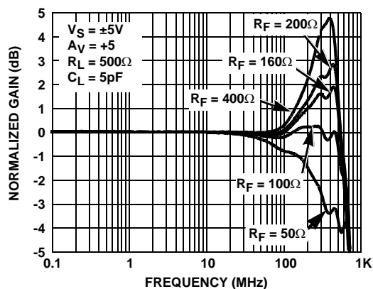
FIGURE 12. GAIN vs FREQUENCY FOR VARIOUS R_F ( A_V = +5 )
