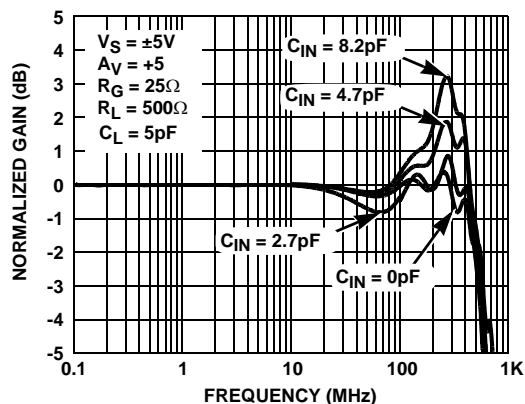
FIGURE 14. GAIN vs FREQUENCY FOR VARIOUS C_{IN(-)} ( A_V = +5 )
