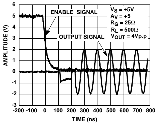
FIGURE 25. TURN-ON TIME
