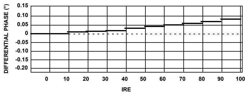
FIGURE 38. DIFFERENTIAL PHASE (°)
