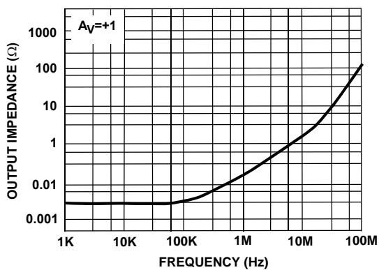
FIGURE 15. OUTPUT IMPEDANCE
