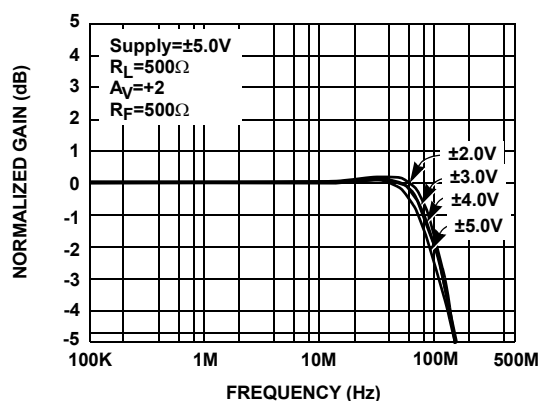
FIGURE 12. FREQUENCY RESPONSE FOR VARIOUS POWER SUPPLY
