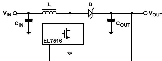
FIGURE 28. BOOST CONVERTER
