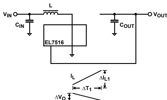
FIGURE 28. BOOST CONVERTER
