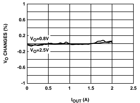
FIGURE 6. LOAD REGULATION @ VIN=3.3V
