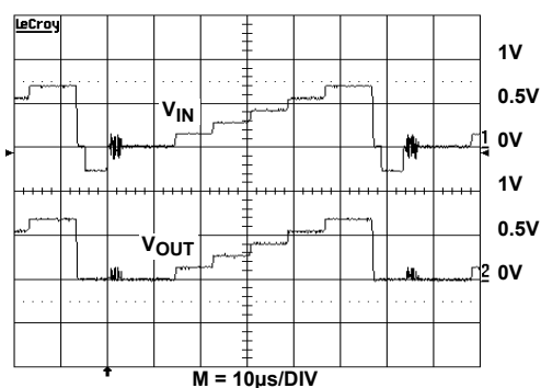
FIGURE 28. VIDEO SIGNAL
