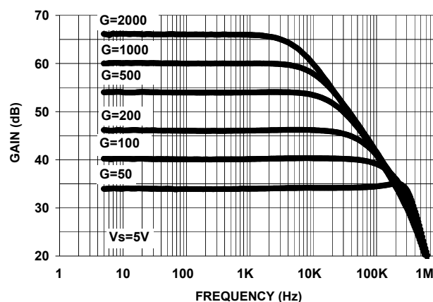
FIGURE 2. EL8172 FREQUENCY RESPONSE vs CLOSED LOOP GAIN
