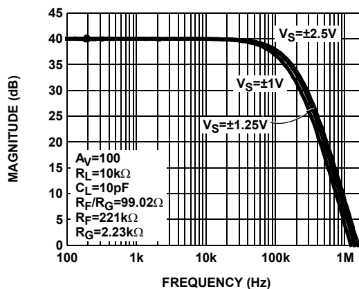
FIGURE 4. EL8172 FREQUENCY RESPONSE vs SUPPLY VOLTAGE
