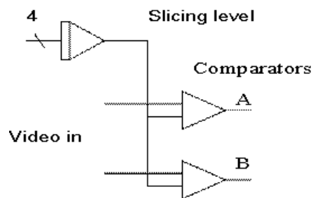
FIGURE 14. DELAY DETECTOR
