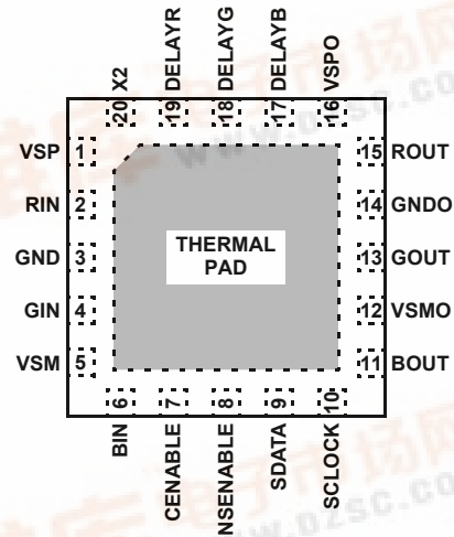
EL9115 [20-PIN QFN (5MM X 5MM)] TOP VIEW
