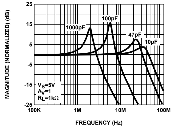
FIGURE 14. FREQUENCY RESPONSE FOR VARIOUS C_L
