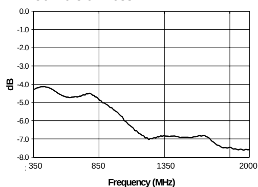
Conversion Loss
