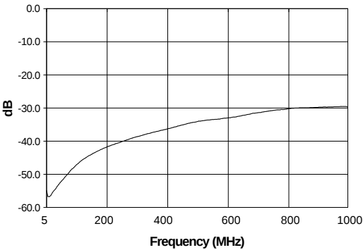
L-R Isolation
