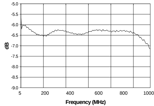
Conversion Loss
