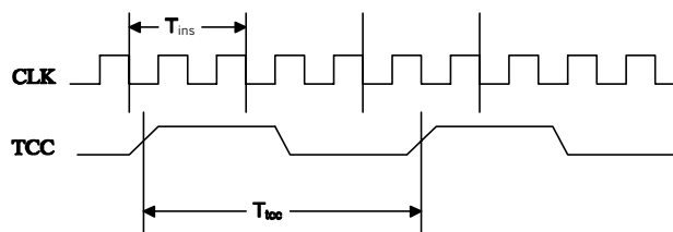
Fig.20 AC timing
