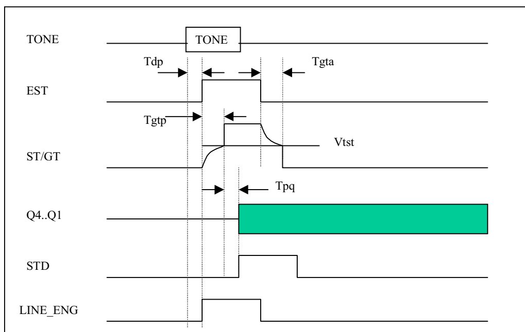
Fig.22. DTMF receiver timing
