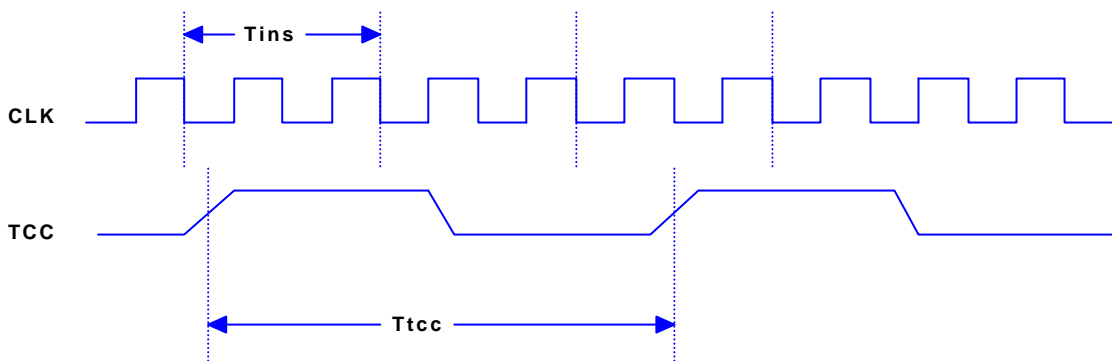
TCC Input Timing (CLKS="0")
