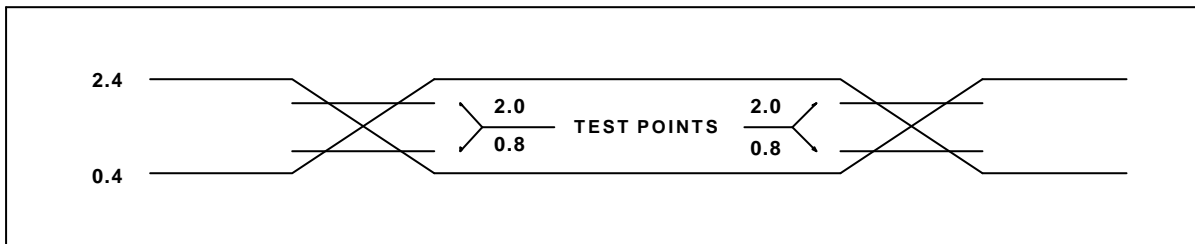
AC Test Input/Output Waveform
