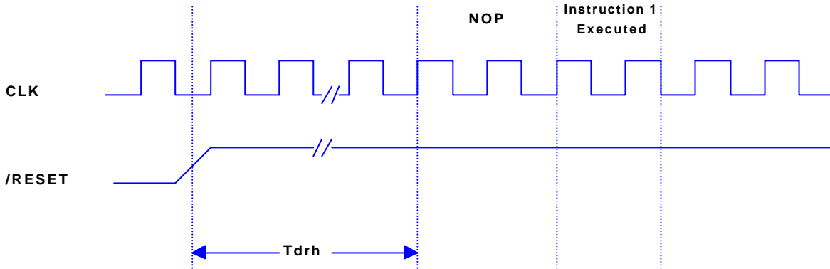
RESET Timing (CLK="0")
