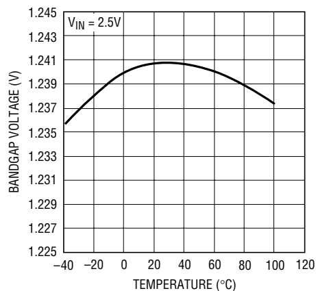
Bandgap Voltage vs Temperature
