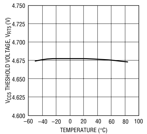
V CC5 Threshold Voltage vs Temperature (LTC1727-5/LTC1728-5)
