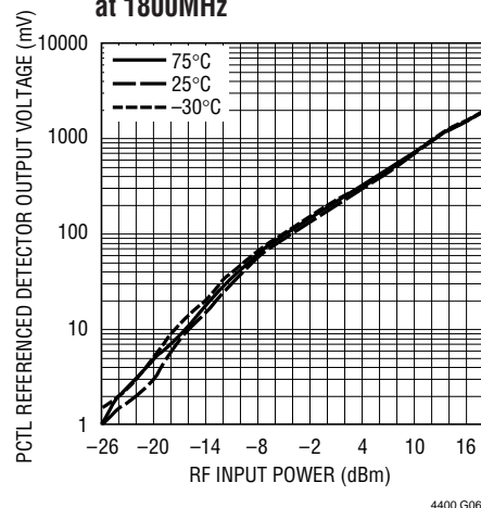
LTC4400-2 Detector Characteristics at 1800MHz
