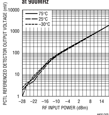
LTC4400-2 Detector Characteristics at 900MHz
