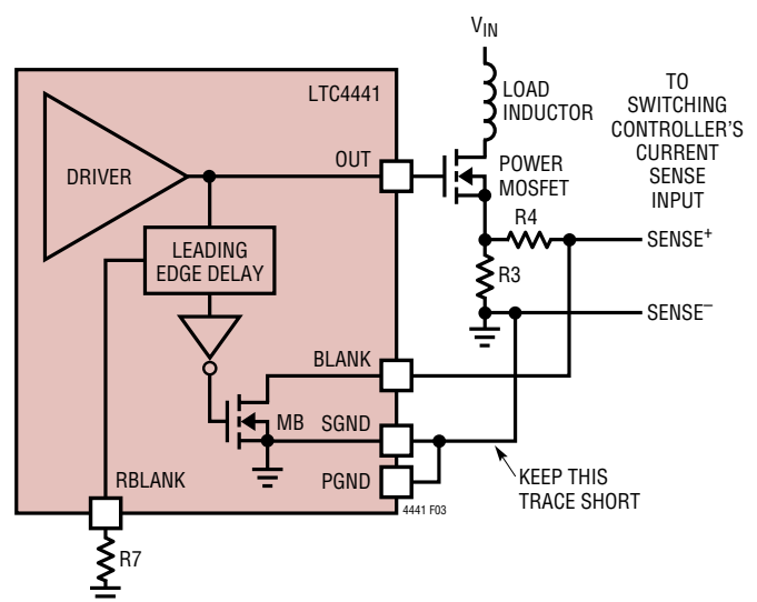
Figure 3. Blanking Circuit
