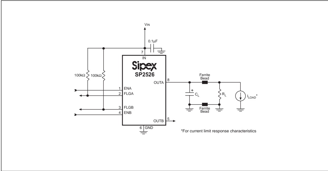
Figure 2. Test Circuit for the SP2526
