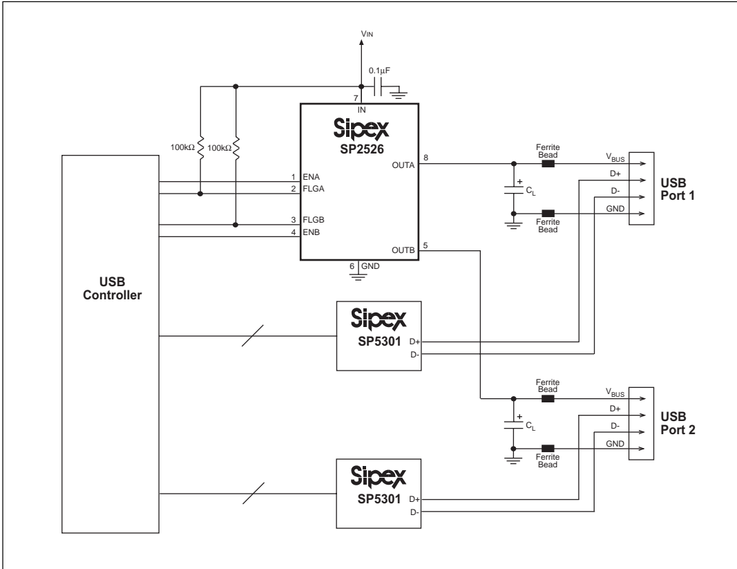
Figure 3. Typical Application Circuit for the SP2526
