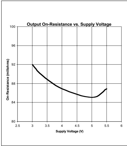
Figure 8. Output On-Resistance vs. Supply Voltage
