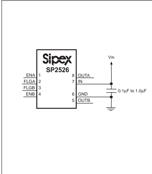
Figure 4. Bypass Capacitor at the Supply Pins
