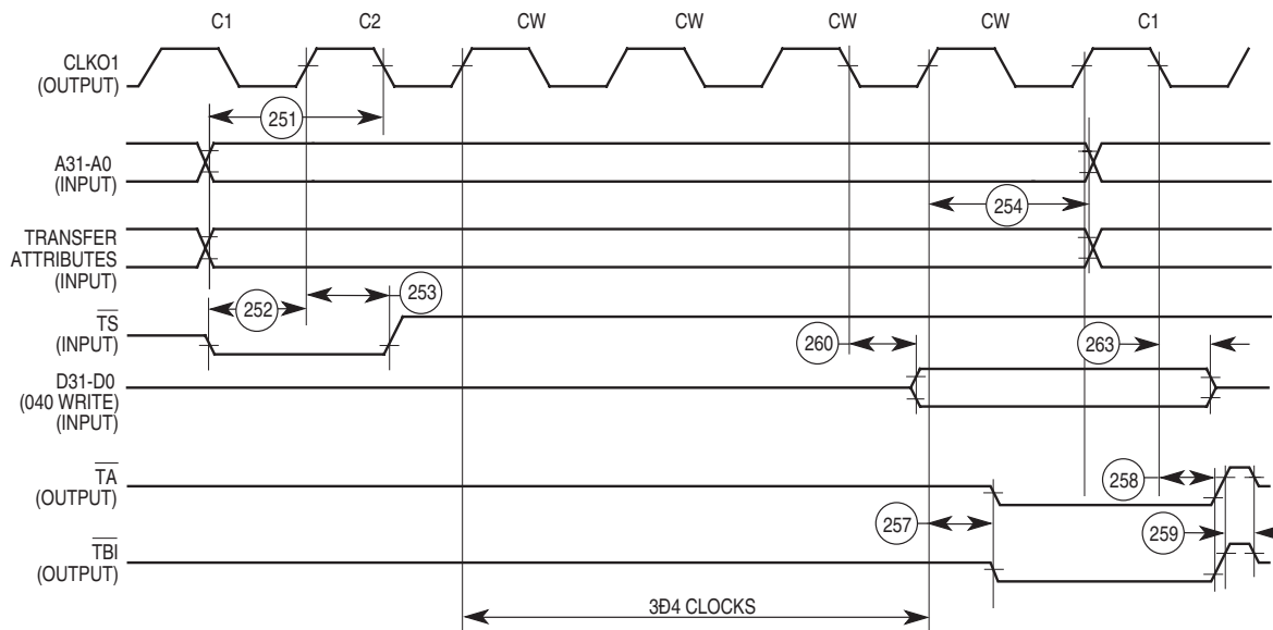
Figure 30. TS68040 Internal Registers Read Cycles
