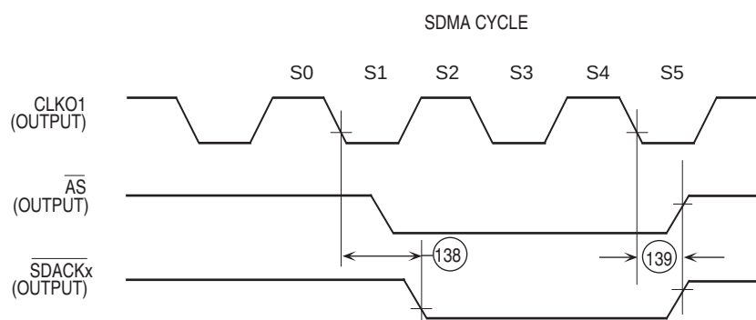
Figure 63. SDACK Timing Diagram
