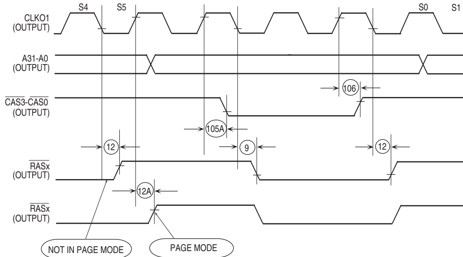
Figure 26. DRAM: Refresh Cycle
