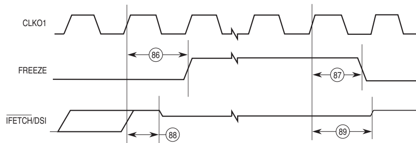
Figure 22. Background Debug Mode FREEZE Timing
