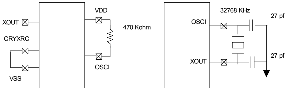
Fig. 15 RC/Crystal OSC Block Diagram
