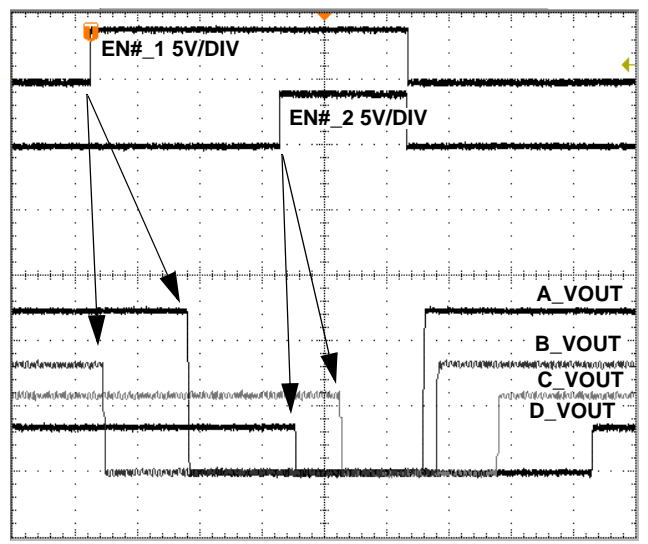
FIGURE 14. ISL6128 GROUP INDEPENDANT TURN-OFF & DELAY ADJUSTABLE PREPROGRAMMED TURN-ON
