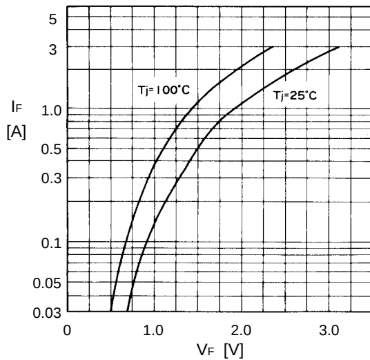
Forward characteristics
