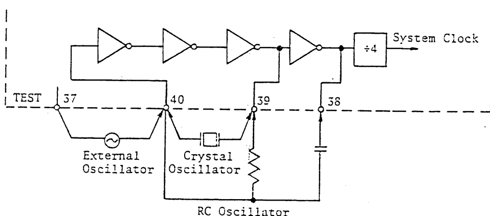
Figure 5: Clock Circuits
