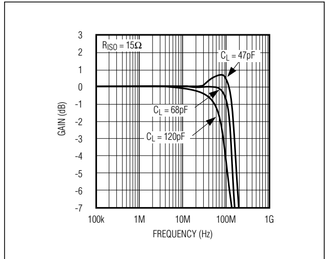
Figure 5. Small-Signal Gain vs. Frequency with Load Capacitance and 15\Omega Isolation Resistor
