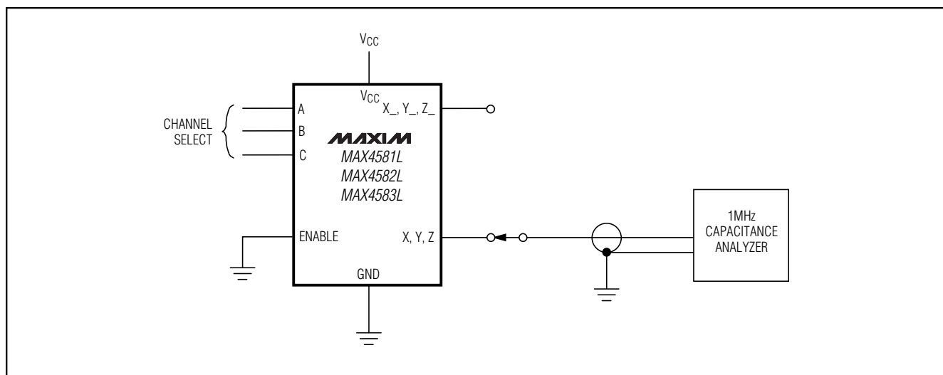
Figure 5. NO/COM Capacitance
