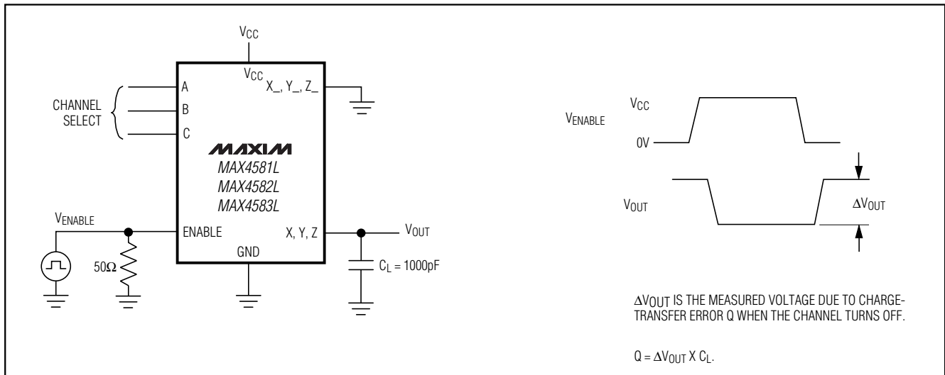
Figure 4. Charge Injection
