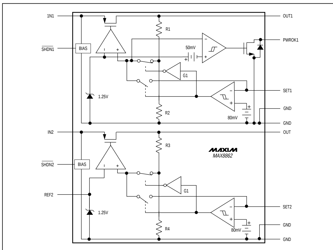
Figure 1. Functional Diagram
