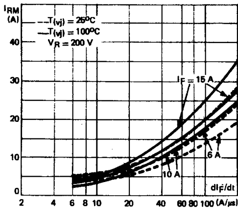
Fig. 9: Peak reverse current versus di_F/dt .
