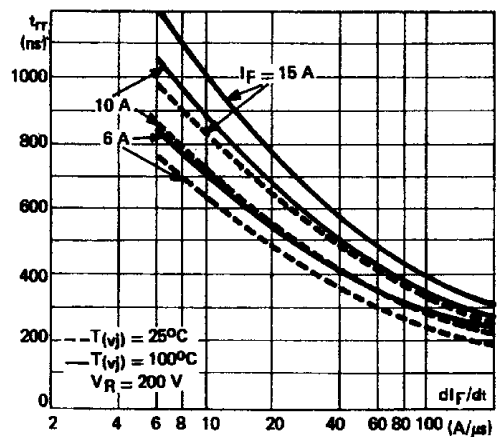
Fig. 8: Recovery time versus di/dt.
