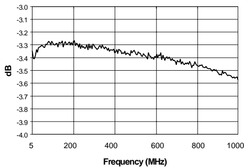
Amplitude Unbalance
