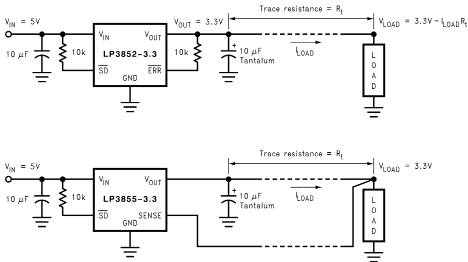
FIGURE 4. Improving remote load regulation using LP3855
