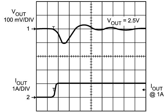
Load Transient Response C_{IN} = 2 \times 10\mu\text{F} CERAMIC C_{OUT} = 2 \times 10\mu\text{F} CERAMIC
