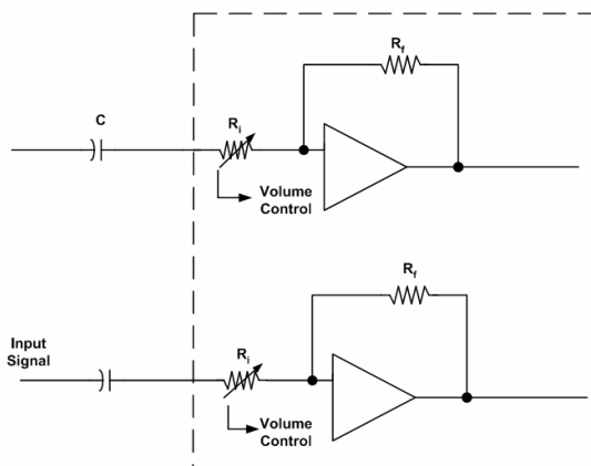
Figure 38. Input Resistor
