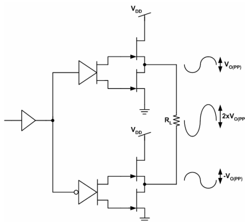
Figure 39. Bridge-Tied Load Configuration
