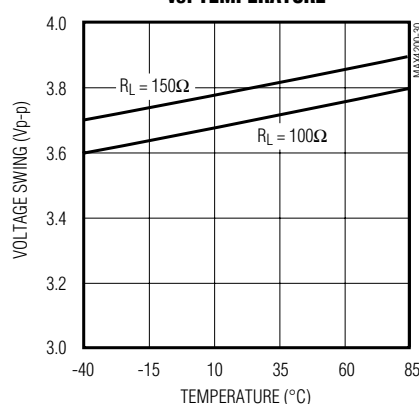
MAX4200/MAX4203 OUTPUT VOLTAGE SWING vs. TEMPERATURE
