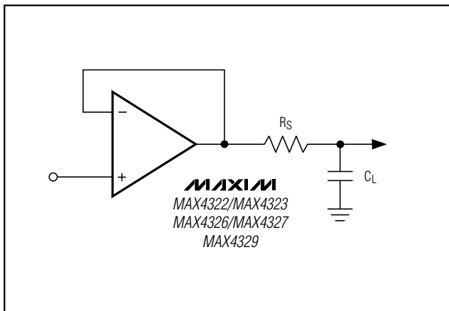
Figure 7. Capacitive-Load-Driving Circuit
