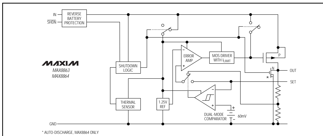
Figure 1. Functional Diagram
