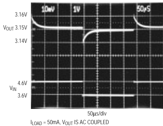
LINE-TRANSIENT RESPONSE
