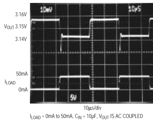
LOAD-TRANSIENT RESPONSE
