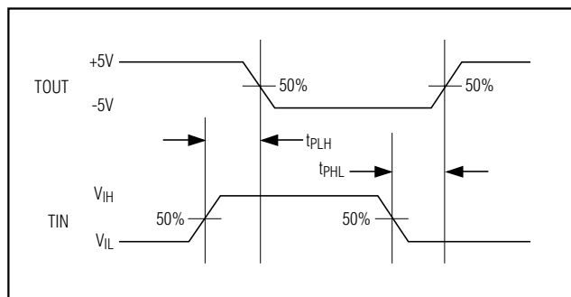
Figure 1. Transmitter Propagation-Delay Timing
