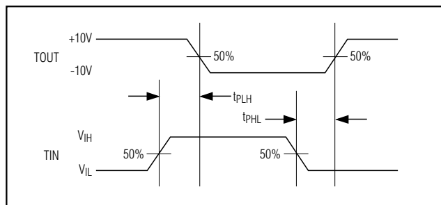
Figure 1. Transmitter Propagation-Delay Timing
