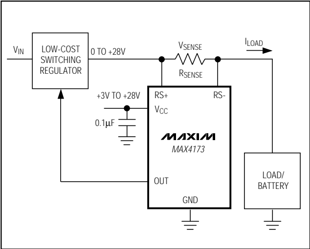
Figure 3. Current Source
