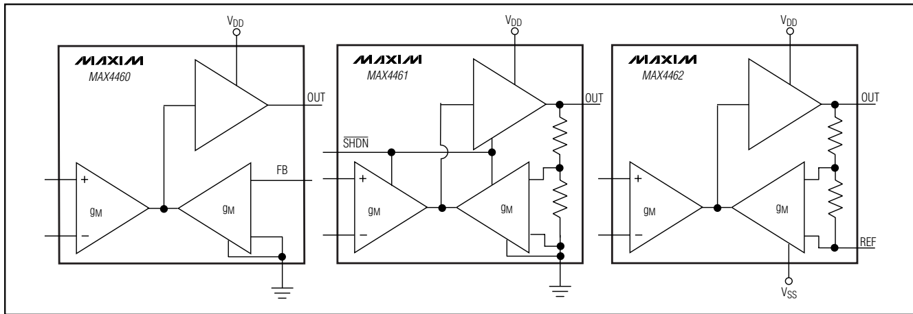
Figure 1. Functional Diagrams
