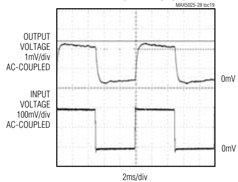
MAX5026, V_{CC} = 5V TO 5.2V , V_{OUT} = 30V , I_{LOAD} = 1mA . CIRCUIT OF FIGURE 2
