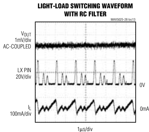
MAX5026, V_{CC} = 5V , V_{OUT} = 30V , I_{LOAD} = 0.1mA . CIRCUIT OF FIGURE 3
