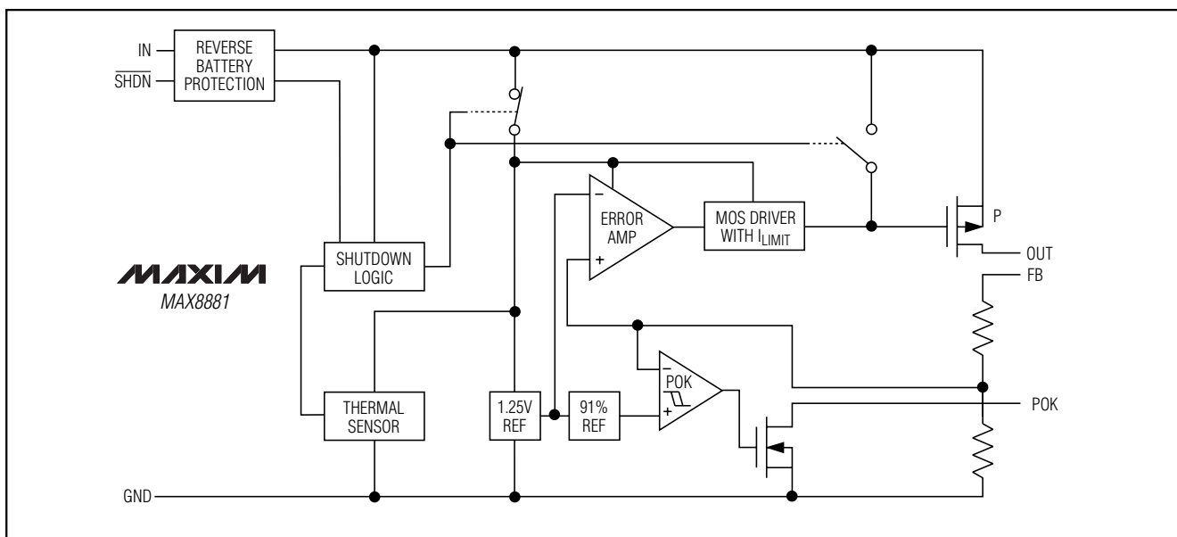
Figure 2. Functional Diagram
