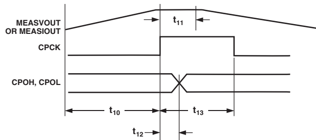
Figure 2. Comparator Timing
