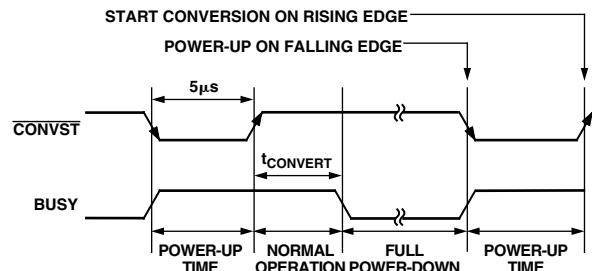
Figure 22. Power-Up Timing When Using \overline{CONVST} Pin
