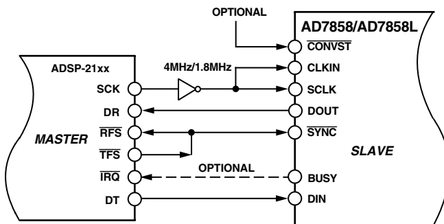
Figure 39. ADSP-21xx Interface
