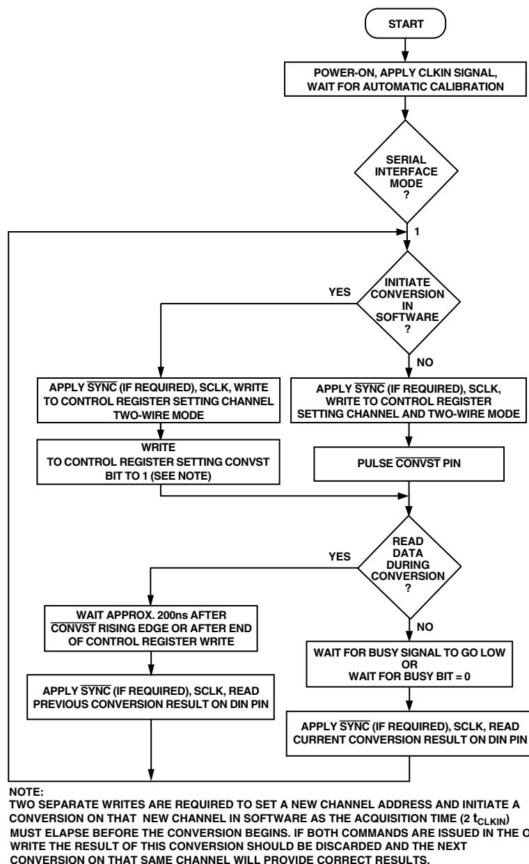
Figure 34. Flowchart for Setting Up, Reading, and Writing in Interface Mode 1
