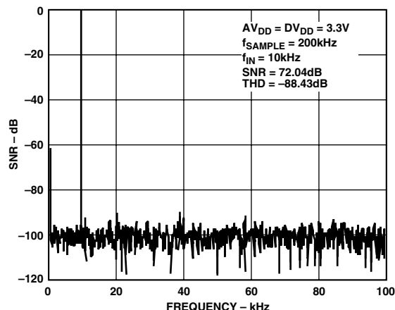
Figure 18. FFT Plot
