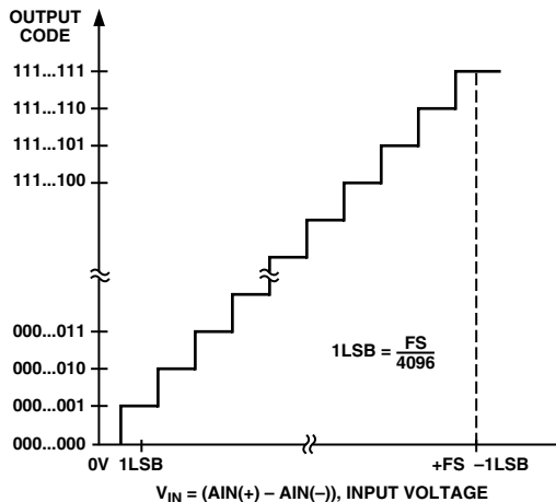
Figure 15. AD7858/AD7858L Transfer Characteristic
