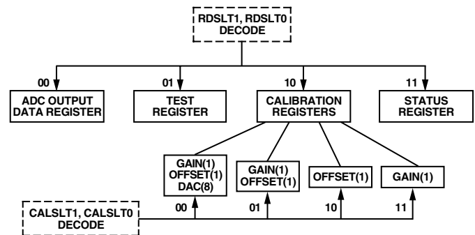
Figure 5. Read Register Hierarchy/Address Decoding
