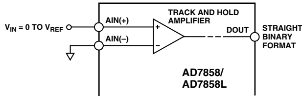
Figure 14. 0 to V_{REF} Input Configuration
