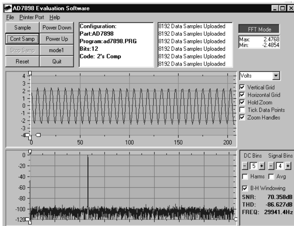
Figure 2. AD7898 Main Screen - FFT Mode
