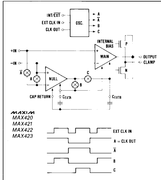
Figure 2. Maxxim MAX420 Series Amplifier Block Diagram.
