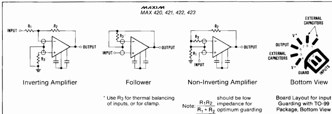
Figure 5. Input Guard Connections.
