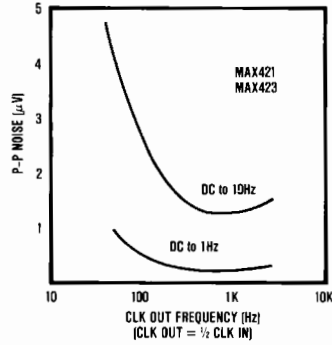
P-P NOISE VOLTAGE vs. CLOCK FREQUENCY
