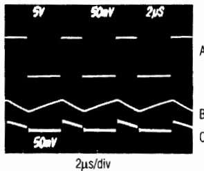
MAX752 SWITCHING WAVEFORMS CONTINUOUS CONDUCTION
