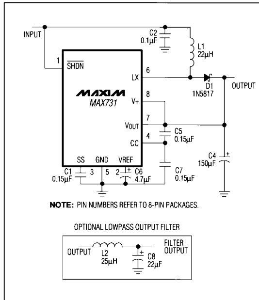
Figure 2a. MAX731 Standard Boost Application Circuit
