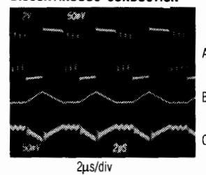
MAX731 SWITCHING WAVEFORMS DISCONTINUOUS CONDUCTION
