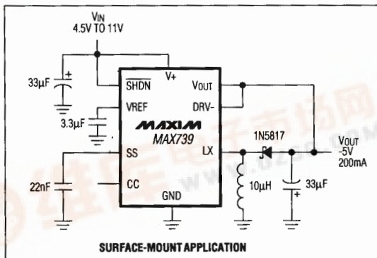
SURFACE-MOUNT APPLICATION
